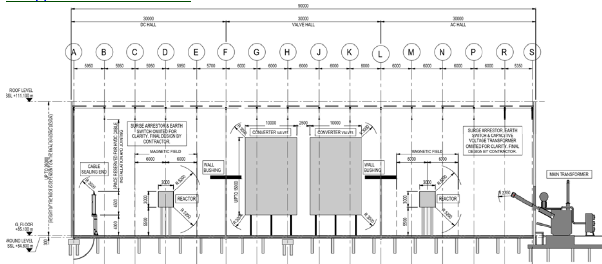
Plate 5.18 – Converter building design Section view 1, extracted from indicative drawing EN020022-X.X-CHLP-Sheet1 in Appendix 1 (not to scale)
