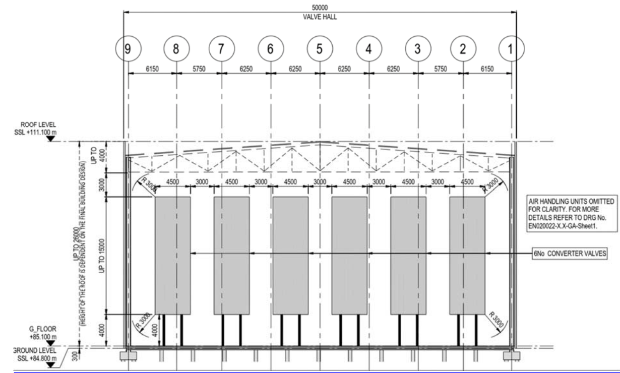
Plate 5.17 – Converter building design Section view 2, extracted from indicative drawing EN020022-X.X-CHLP-Sheet1 in Appendix 1 (not to scale)
